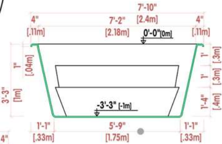
CORTE TRANSVERSAL |CROSS SECTION|LA COUPE TRANSVERSALE
